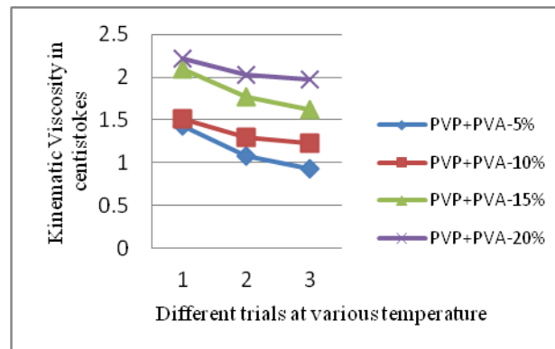
Figure 5.3: Kinematic Viscosity of PVP and PVA
