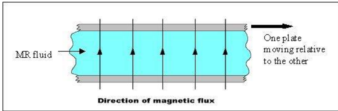
Fig 1.3- Shear mode
