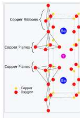
Fig. 5 Crystal structure of Y-Ba-Cu-O
