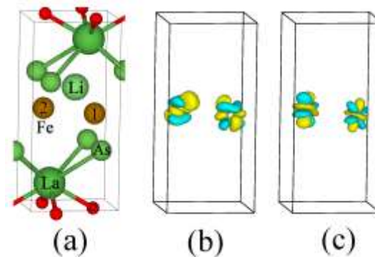
Fig. 7 (a) Crystal structure of LaFeAsO; (b) charge density change caused by insertion of a \text{Li}^+ ion; (c) charge density change caused by a uniform electric field (yellow indicates increased charge density, blue decreases)
