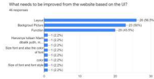
Figure 7. Users responses
