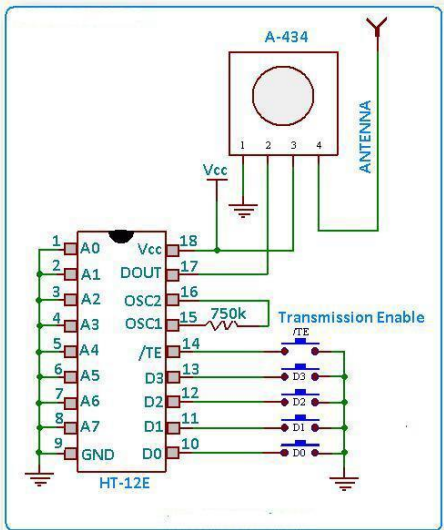
FIG 1: RF Trasmmitter Module
