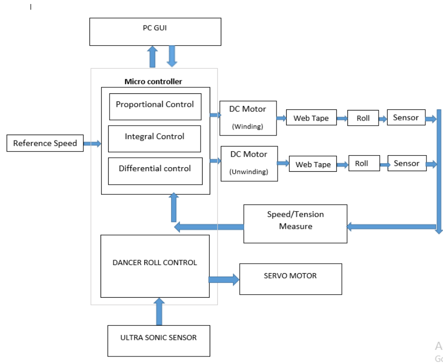
Figure 2. Block Diagram of Proposed Idea
