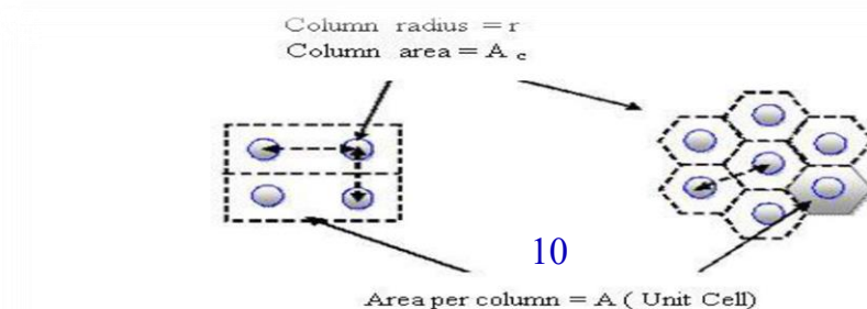
Figure: 1 Plan of stone column, Square pattern and Triangular pattern (Cabe,2007)
