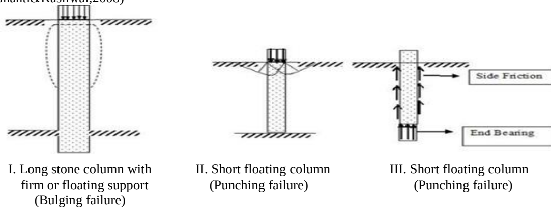
Figure 2: Failure mechanism of a single stone column in a homogeneous soft layer (Ghanti&Kasliwal,2008)
