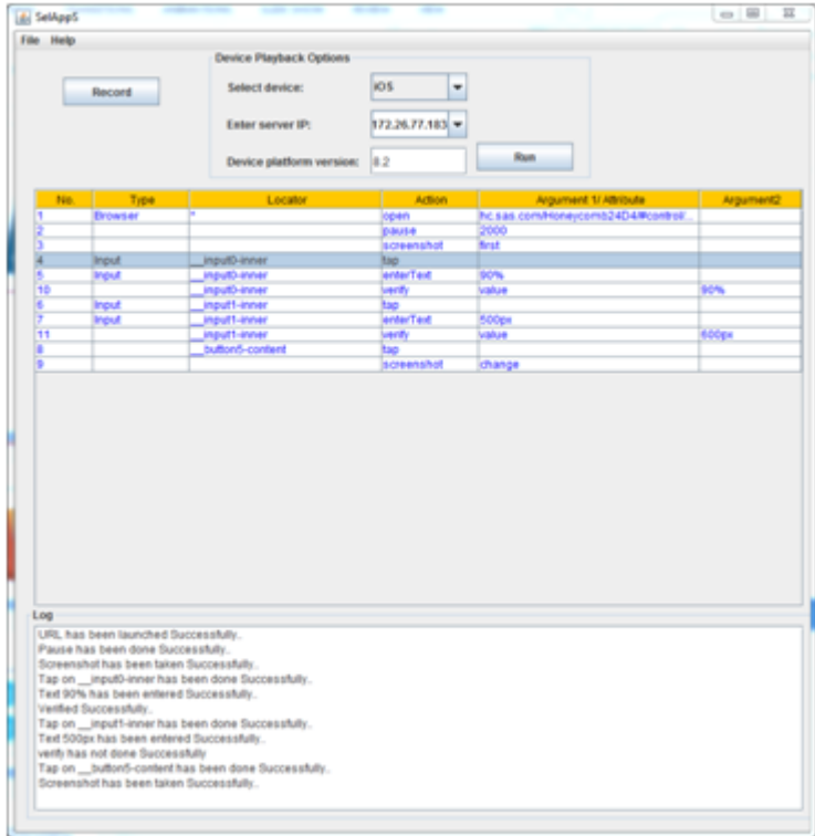
Figure 3: Running test case and log generation
