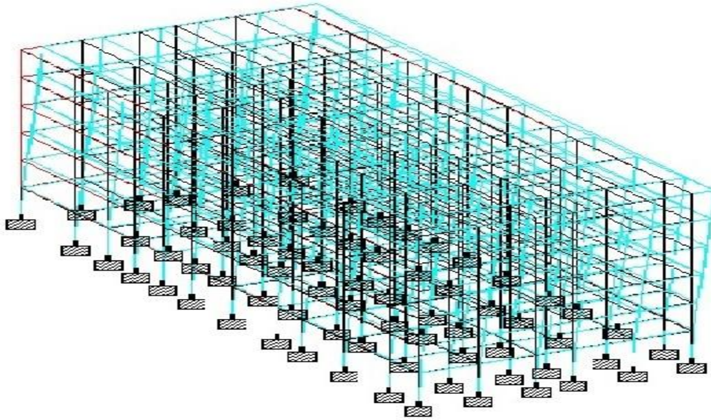
Fig 10 Deflection diagram
