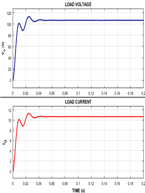
Figure 10: Voltage across load and current through load for converter operation in boost mode
